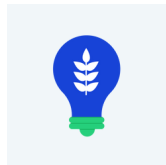
Energy
